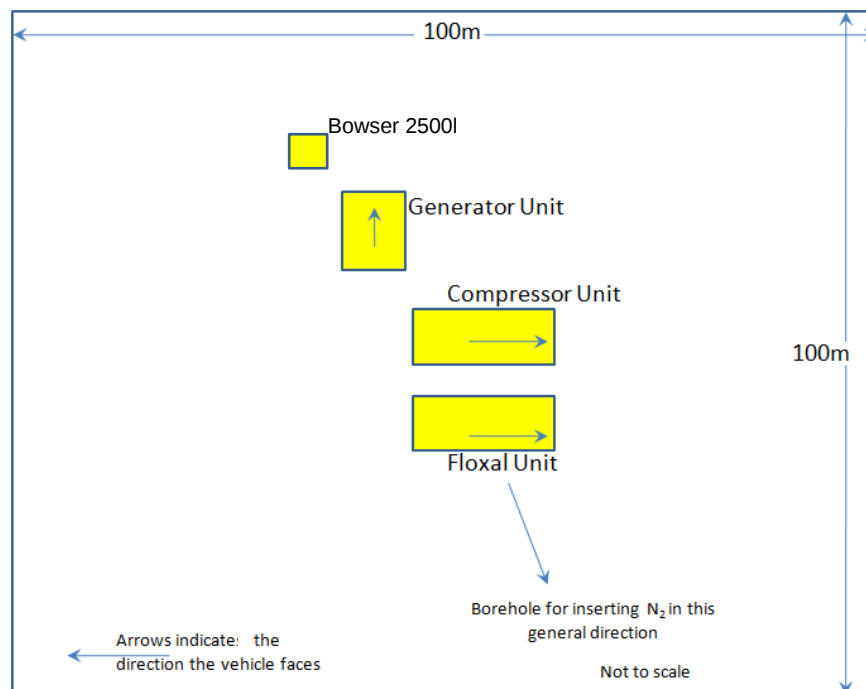
Figure 3: CIS General layout. Please note that the T685WS drill (as sketched below) may be deployed anywhere within the boundary indicated above.
