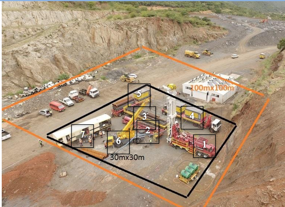
Figure 1: Typical arrangement of vehicles when RDU is deployed.
